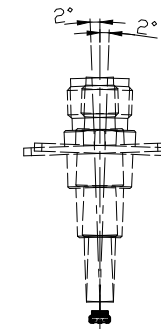
MATING ANGLE
