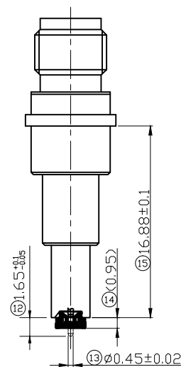
MATED CONDITION
